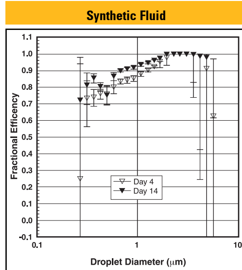
Efficiency vs. droplet diameter for Dryflo cartridge and wrap assembly on days 4 and 14 with synthetic fluid at an airflow of 1000 CFM. Error bars represent 95% confidence intervals.
