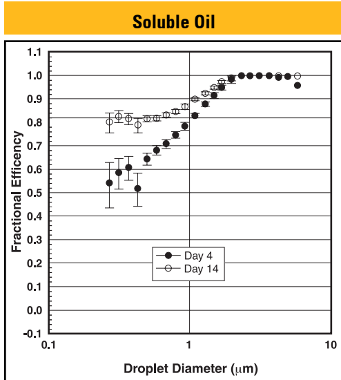
Efficiency vs. droplet diameter for Dryflo cartridge and wrap assembly on days 4 and 14 with soluble oil at an airflow of 1000 CFM. Error bars represent 95% confidence intervals.
